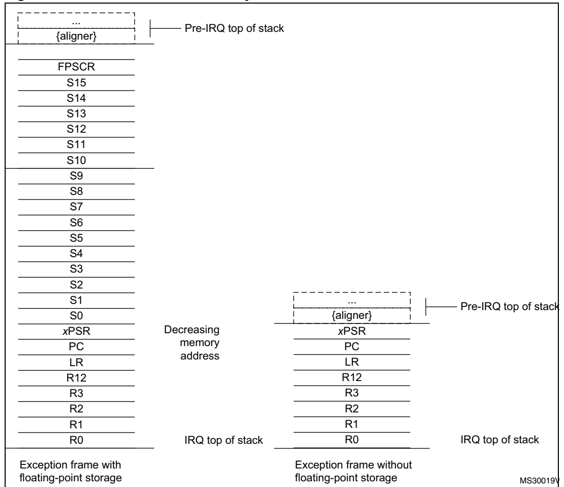
Figure 12. Cortex-M4 stack frame layout
