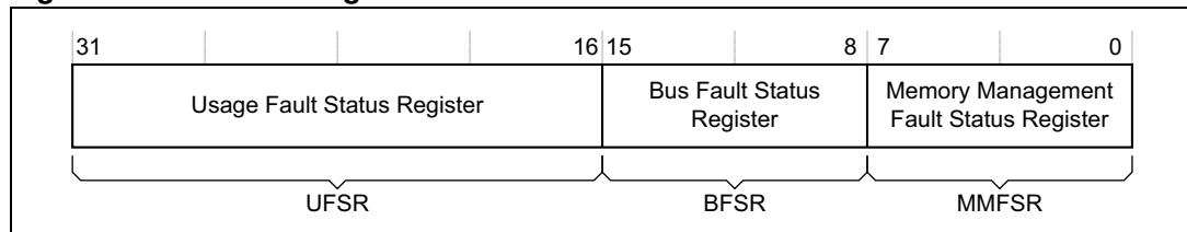
Figure 20. CFSR subregisters
