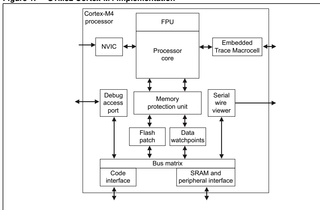
Figure 1. STM32 Cortex-M4 implementation
