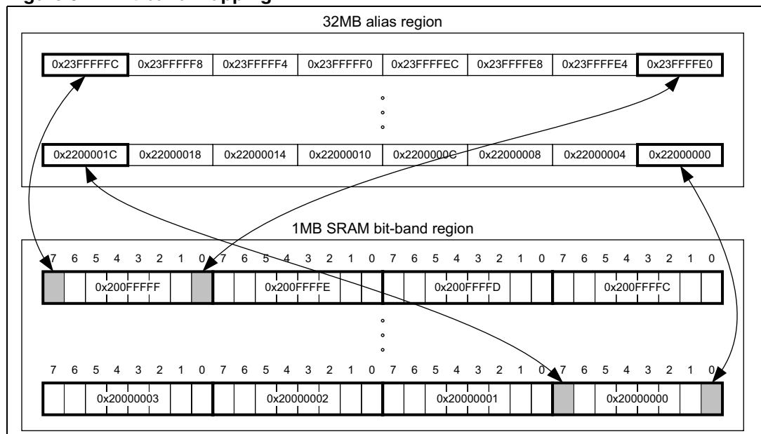
Figure 9. Bit-band mapping
